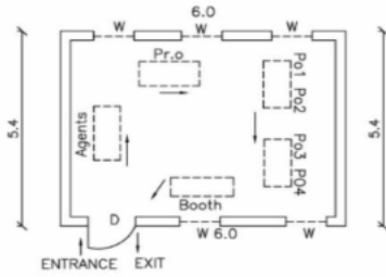
CAD Drawing.
