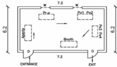
CAD Drawing.
