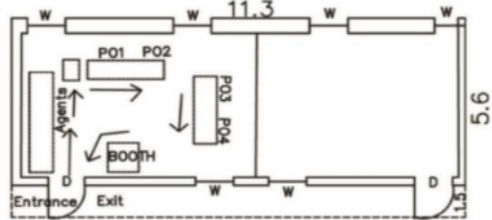
(3) CAD Drawing
