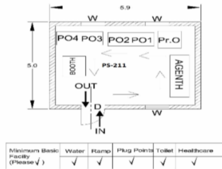
Cad View
