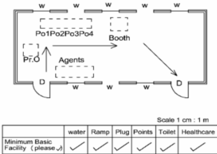
CAD Drawing
