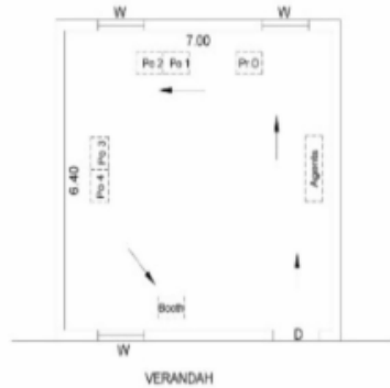
(3) CAD Drawing
