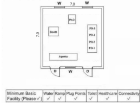
3. Cad Drawing
