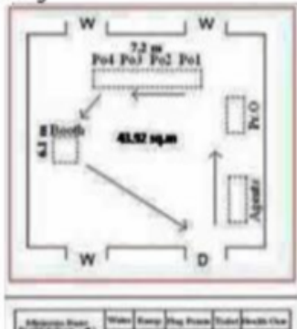
3. CAD Drawing
