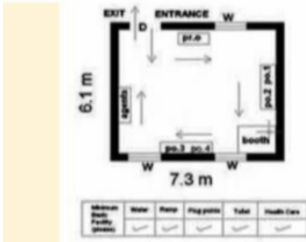
3. CAD Drawing
