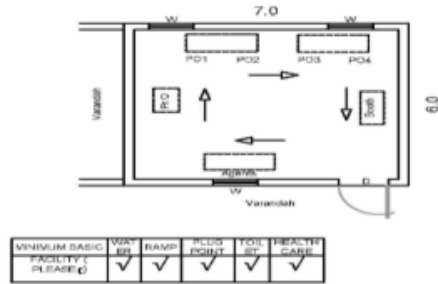
(3) CAD DRAWING
