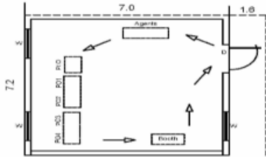
(3) CAD DRAWING
