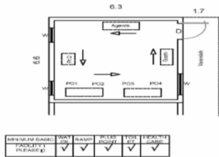
(3) CAD DRAWING
