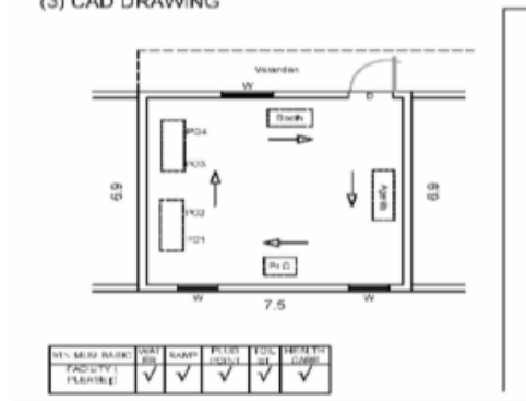
(3) CAD DRAWING
