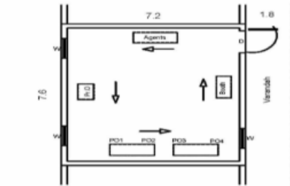
(3) CAD DRAWING ELEVATION
