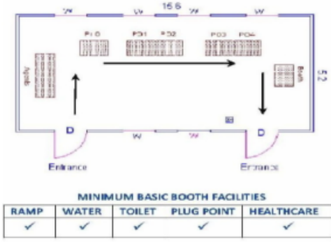
3. CAD Drawing
