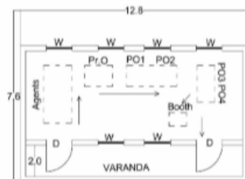
Cad View
