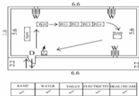
(3) CAD Drawing
