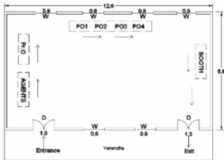
Cad View
