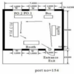
CAD Drawing
