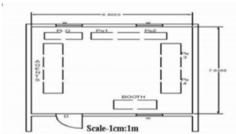
CAD Drawing
