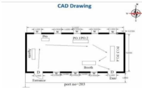
Cad View
