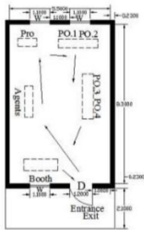
CAD Drawing
