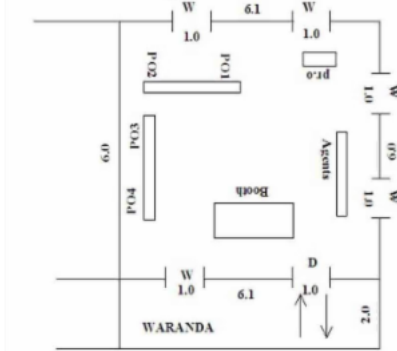
Cad Drawing
