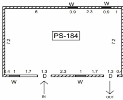
CAD DRAWING
