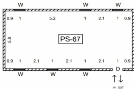
CAD DRAWING
