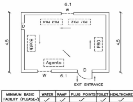
CAD Drawing.
