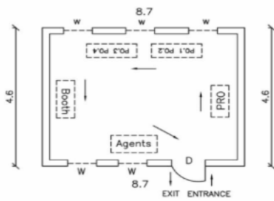
CAD Drawing.
