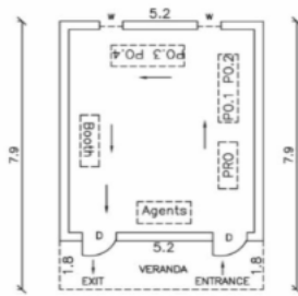
CAD Drawing.
