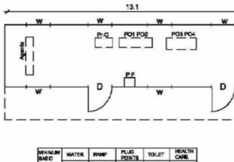
(3) CAD Drawing
