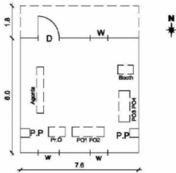
(3) CAD Drawing
