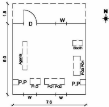
(3) CAD Drawing
