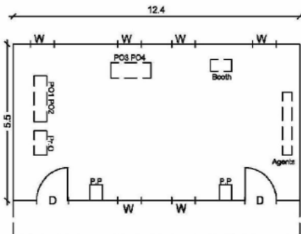
(3) CAD Drawing
