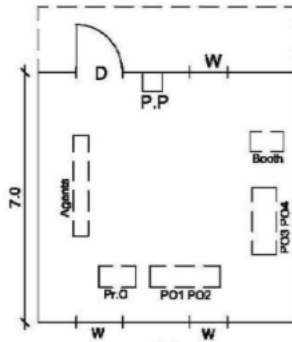
(3) CAD Drawing
