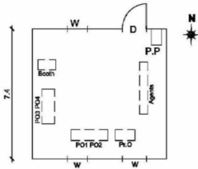
(3) CAD Drawing
