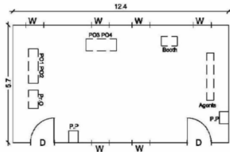
(3) CAD Drawing
