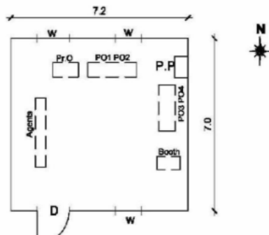
(3) CAD Drawing
