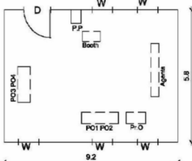
(3) CAD Drawing
