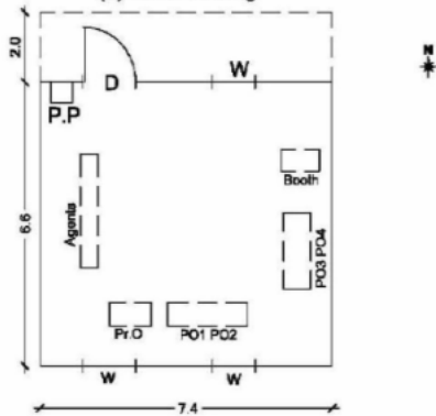
(3) CAD Drawing
