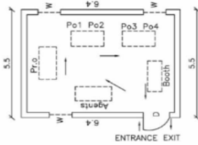
CAD Drawing.
