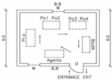
CAD Drawing.
