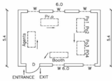
CAD Drawing.
