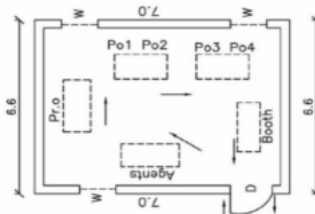
CAD Drawing.
