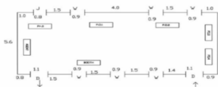
CAD Drawing.
