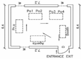
CAD Drawing.
