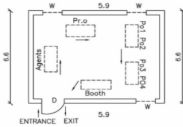
CAD Drawing.
