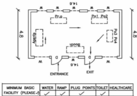
CAD Drawing.
