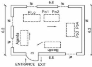
CAD Drawing.
