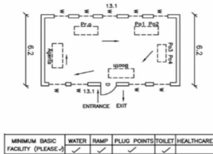
CAD Drawing.
