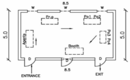
CAD Drawing.
