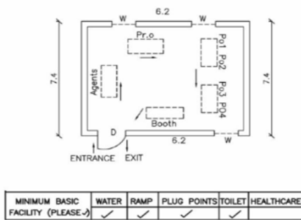
CAD Drawing.
